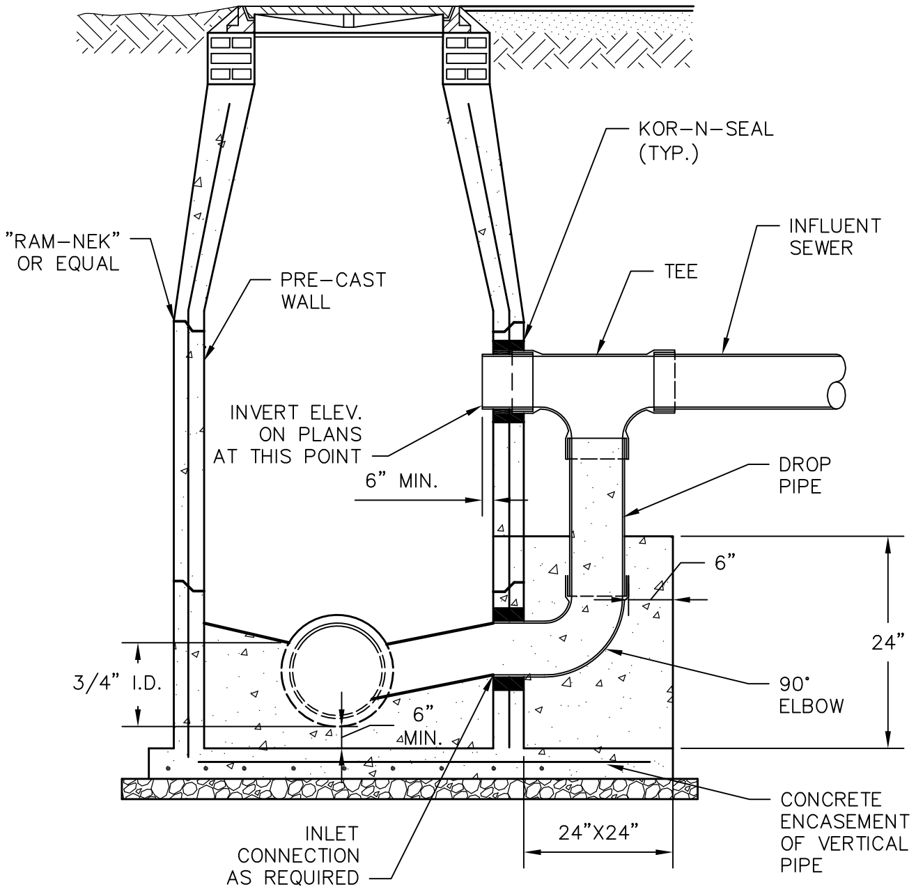
SECTION VIEW
